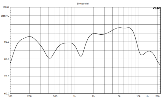
Frequency Response
