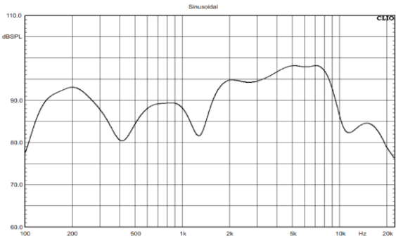
Frequency Response
