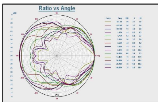
Polar Diagram
