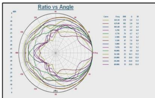
Polar Diagram
